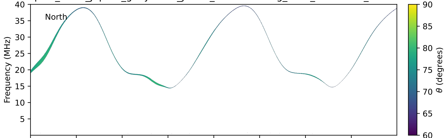
expres_earth_jupiter_ganymede_jrm33_lossc-wid1deg_3kev_20180317_v11.cdf
