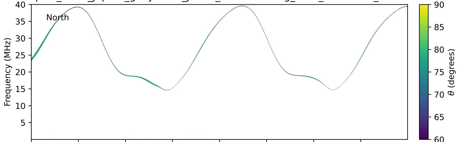
expres_earth_jupiter_ganymede_jrm33_lossc-wid1deg_3kev_20180310_v11.cdf
