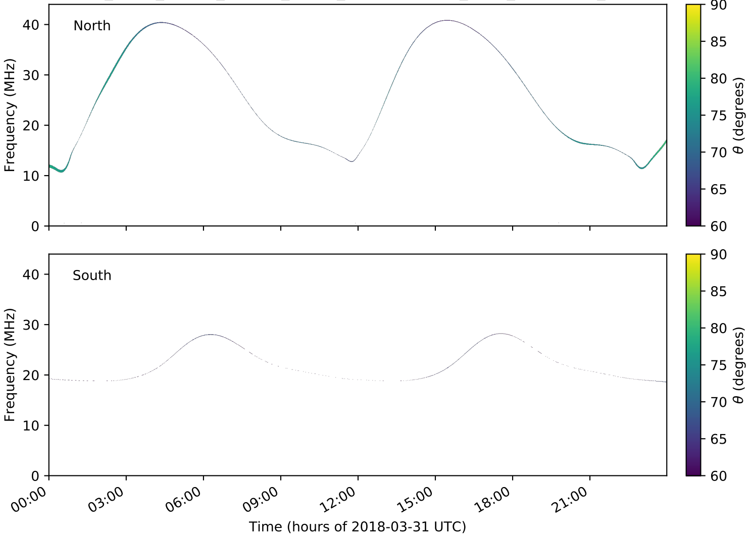
expres_earth_jupiter_europa_jrm09_lossc-wid1deg_3kev_20180331_v01.cdf
