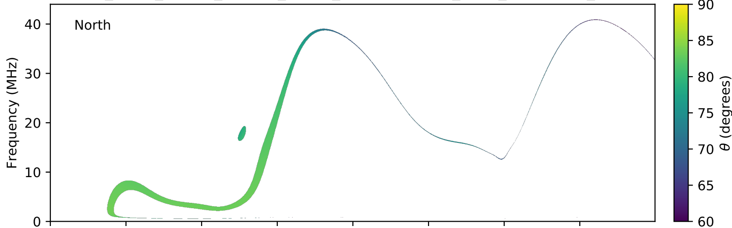
expres_earth_jupiter_europa_jrm09_lossc-wid1deg_3kev_20180327_v01.cdf
