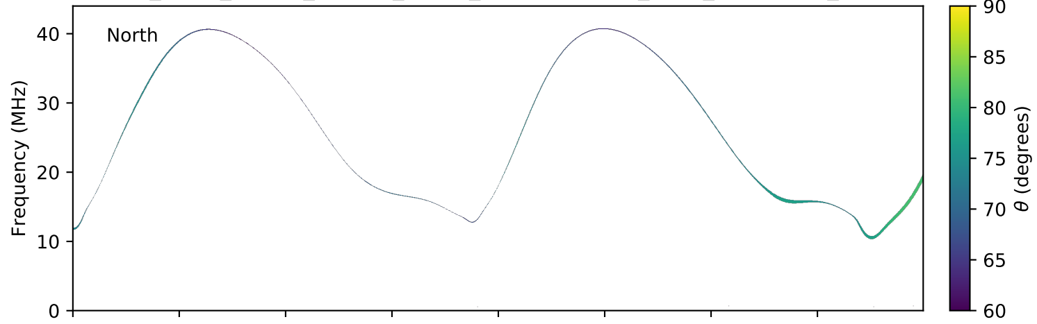
expres_earth_jupiter_europa_jrm09_lossc-wid1deg_3kev_20180324_v01.cdf
