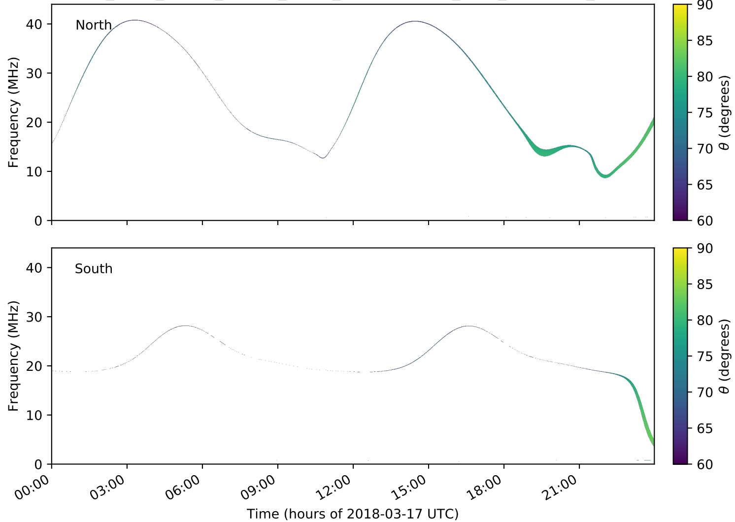
expres_earth_jupiter_europa_jrm09_lossc-wid1deg_3kev_20180317_v01.cdf
