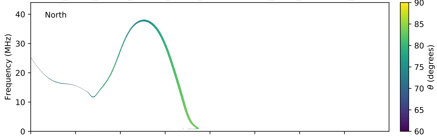
expres_earth_jupiter_europa_jrm09_lossc-wid1deg_3kev_20180314_v01.cdf
