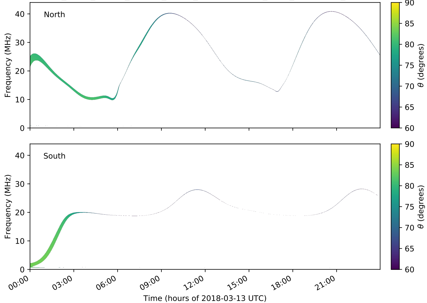
expres_earth_jupiter_europa_jrm09_lossc-wid1deg_3kev_20180313_v01.cdf
