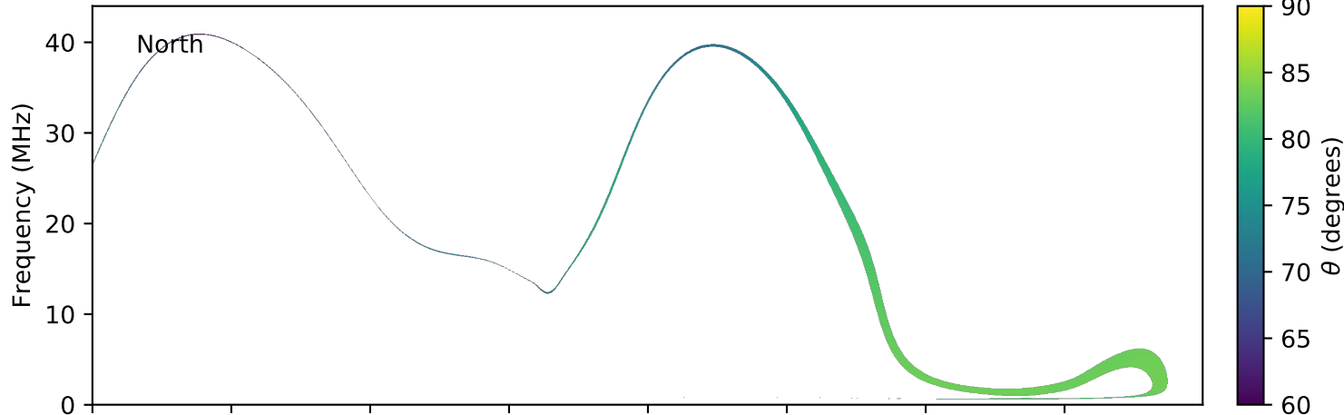
expres_earth_jupiter_europa_jrm09_lossc-wid1deg_3kev_20180303_v01.cdf
