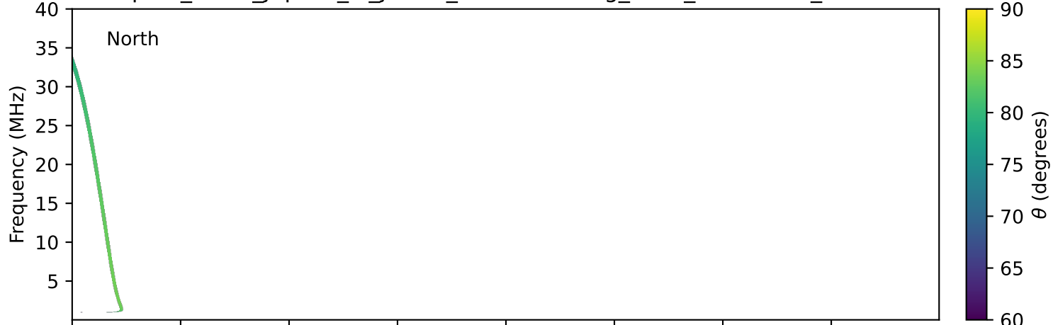
expres_earth_jupiter_io_jrm33_lossc-wid1deg_3kev_20180225_v11.cdf
