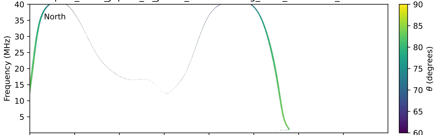
expres_earth_jupiter_io_jrm33_lossc-wid1deg_3kev_20180219_v11.cdf
