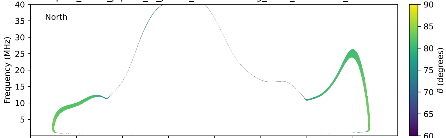
expres_earth_jupiter_io_jrm33_lossc-wid1deg_3kev_20180210_v11.cdf
