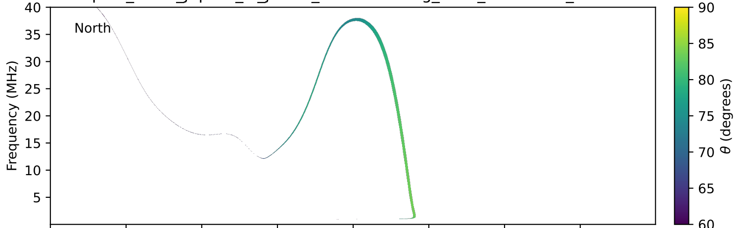
expres_earth_jupiter_io_jrm33_lossc-wid1deg_3kev_20180205_v11.cdf
