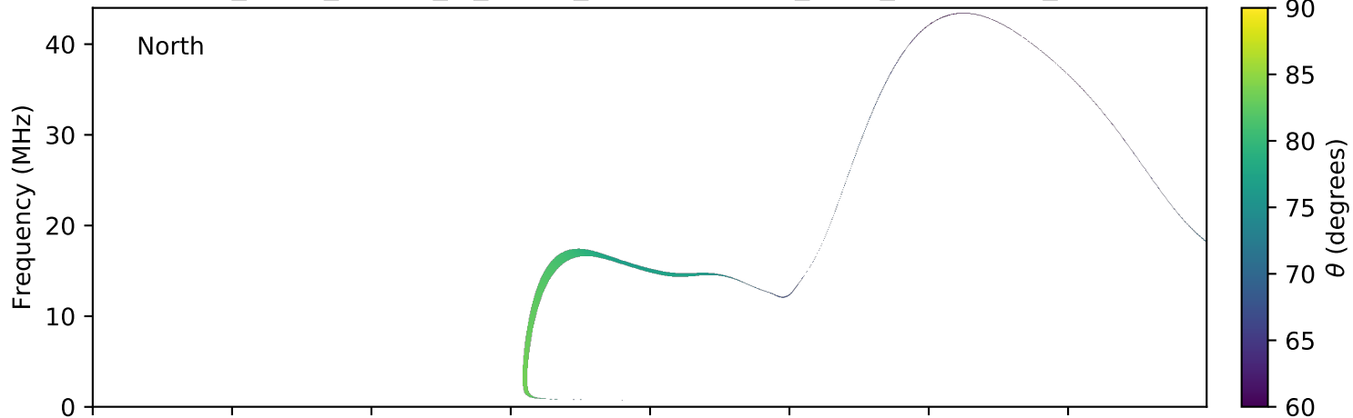
expres_earth_jupiter_io_jrm09_lossc-wid1deg_3kev_20180215_v01.cdf
