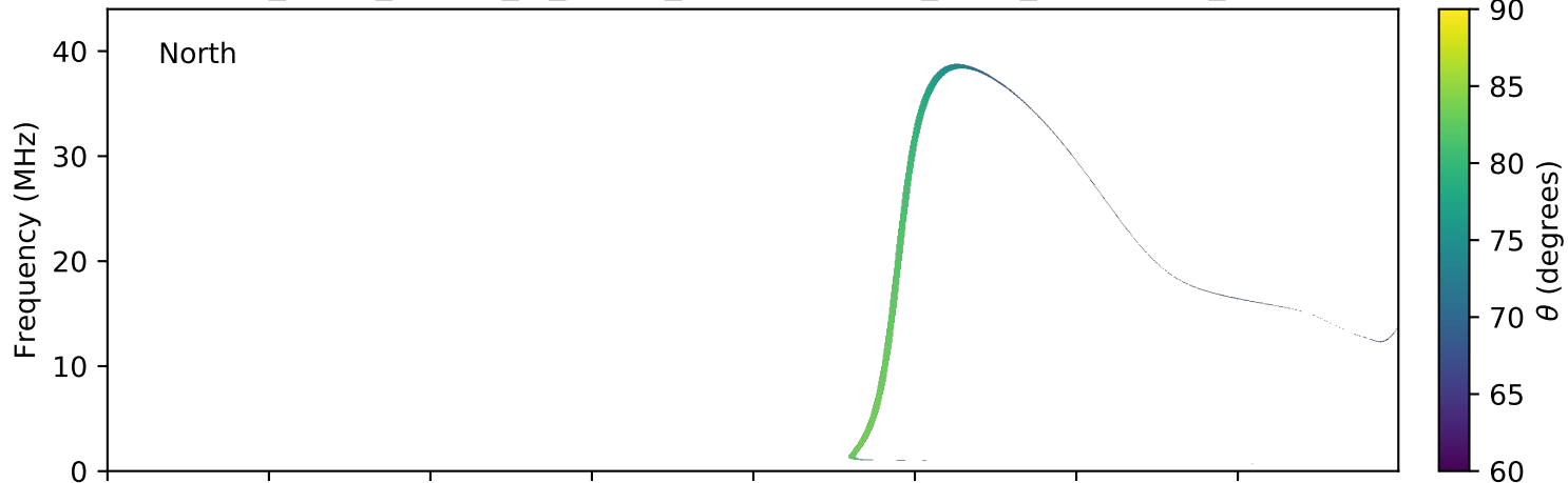
expres_earth_jupiter_io_jrm09_lossc-wid1deg_3kev_20180206_v01.cdf
