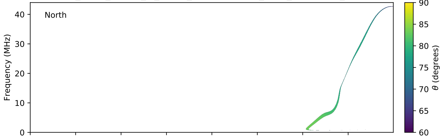
expres_earth_jupiter_io_jrm09_lossc-wid1deg_3kev_20180204_v01.cdf
