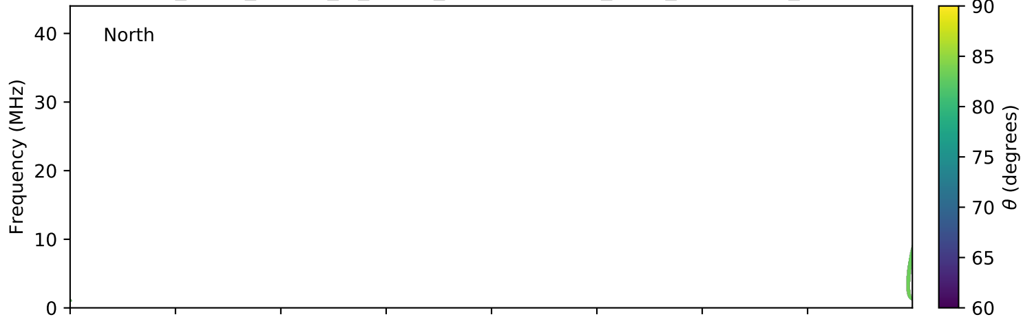
expres_earth_jupiter_io_jrm09_lossc-wid1deg_3kev_20180202_v01.cdf
