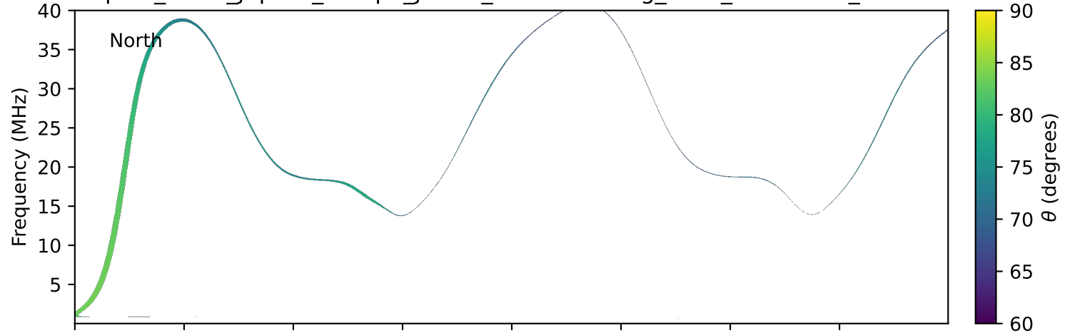
expres_earth_jupiter_europa_jrm33_lossc-wid1deg_3kev_20180202_v11.cdf
