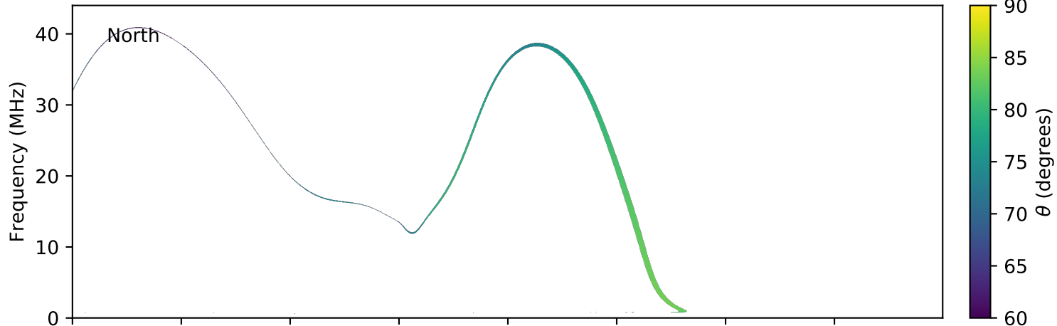
expres_earth_jupiter_europa_jrm09_lossc-wid1deg_3kev_20180224_v01.cdf
