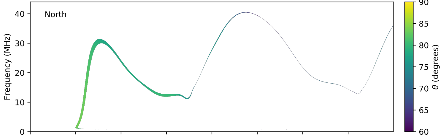
expres_earth_jupiter_europa_jrm09_lossc-wid1deg_3kev_20180216_v01.cdf
