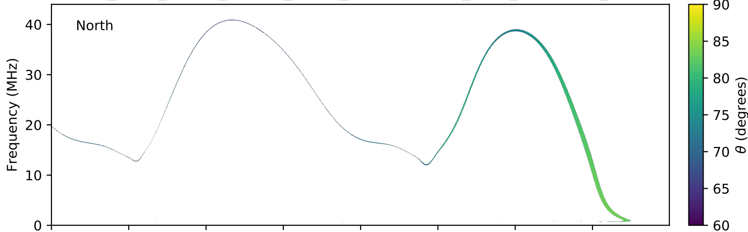
expres_earth_jupiter_europa_jrm09_lossc-wid1deg_3kev_20180206_v01.cdf
