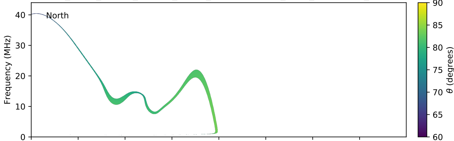
expres_earth_jupiter_europa_jrm09_lossc-wid1deg_3kev_20180203_v01.cdf
