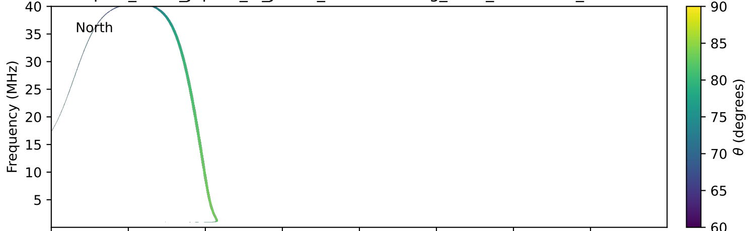
expres_earth_jupiter_io_jrm33_lossc-wid1deg_3kev_20180131_v11.cdf
