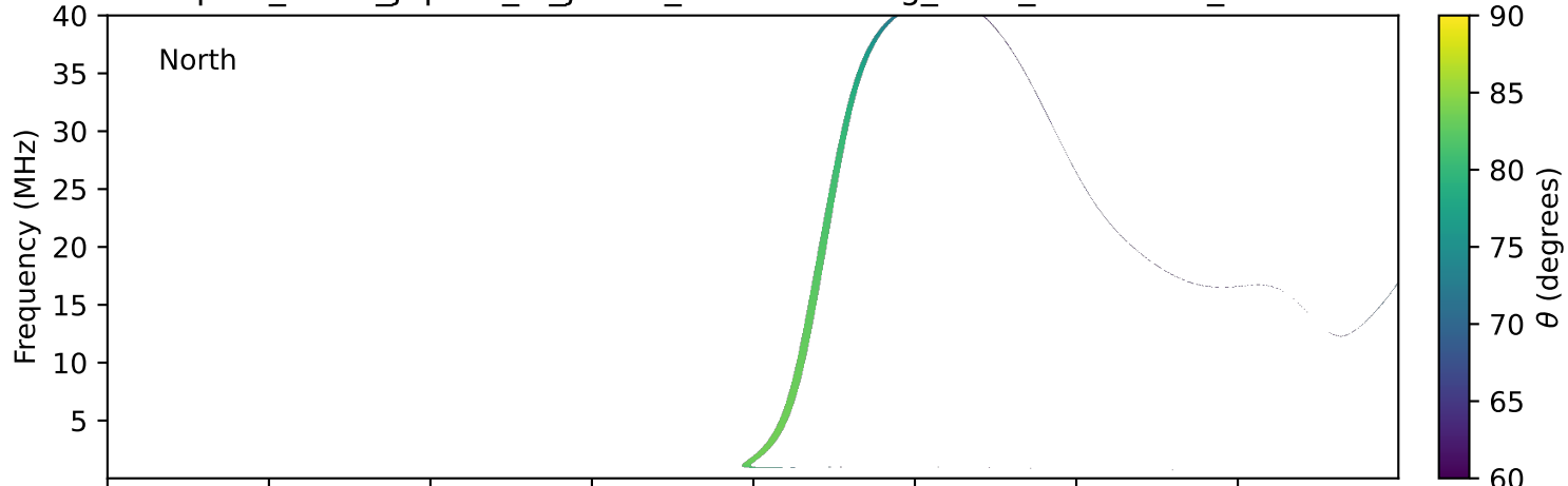
expres_earth_jupiter_io_jrm33_lossc-wid1deg_3kev_20180130_v11.cdf
