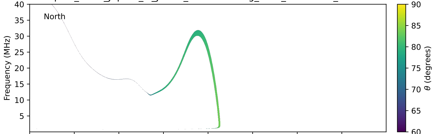
expres_earth_jupiter_io_jrm33_lossc-wid1deg_3kev_20180129_v11.cdf
