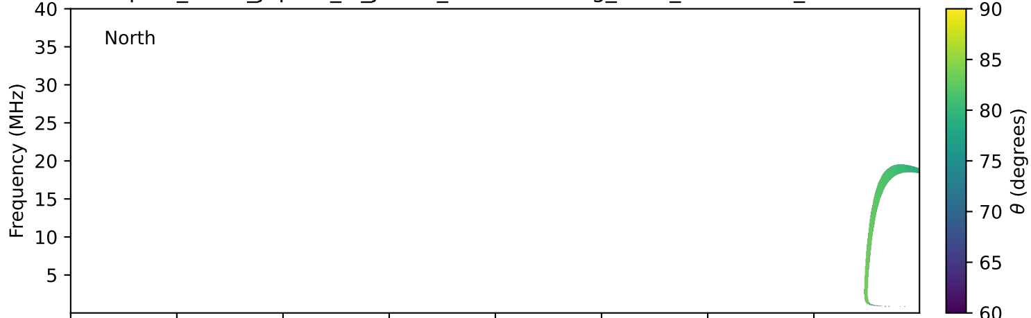
expres_earth_jupiter_io_jrm33_lossc-wid1deg_3kev_20180126_v11.cdf
