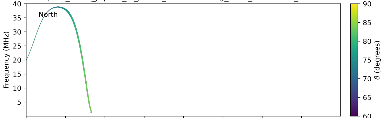
expres_earth_jupiter_io_jrm33_lossc-wid1deg_3kev_20180124_v11.cdf
