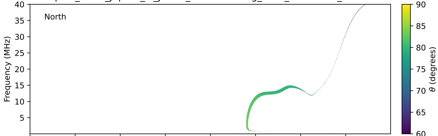
expres_earth_jupiter_io_jrm33_lossc-wid1deg_3kev_20180121_v11.cdf
