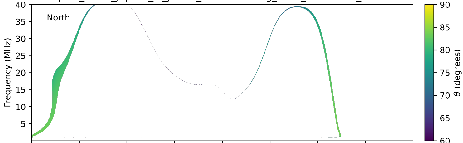
expres_earth_jupiter_io_jrm33_lossc-wid1deg_3kev_20180111_v11.cdf
