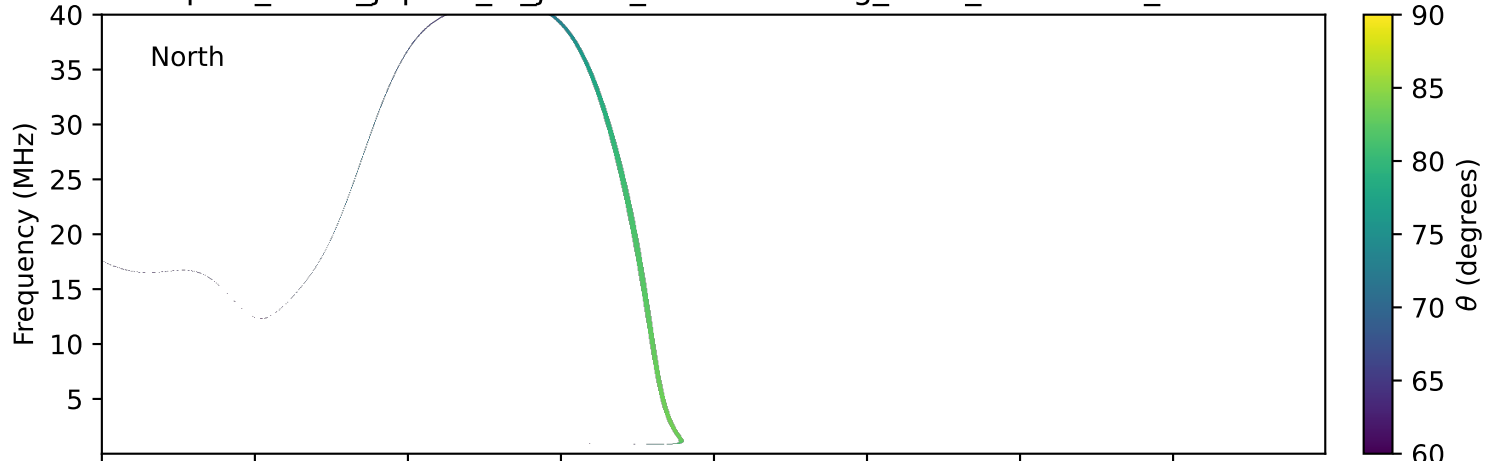
expres_earth_jupiter_io_jrm33_lossc-wid1deg_3kev_20180106_v11.cdf
