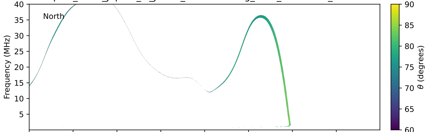
expres_earth_jupiter_io_jrm33_lossc-wid1deg_3kev_20180104_v11.cdf
