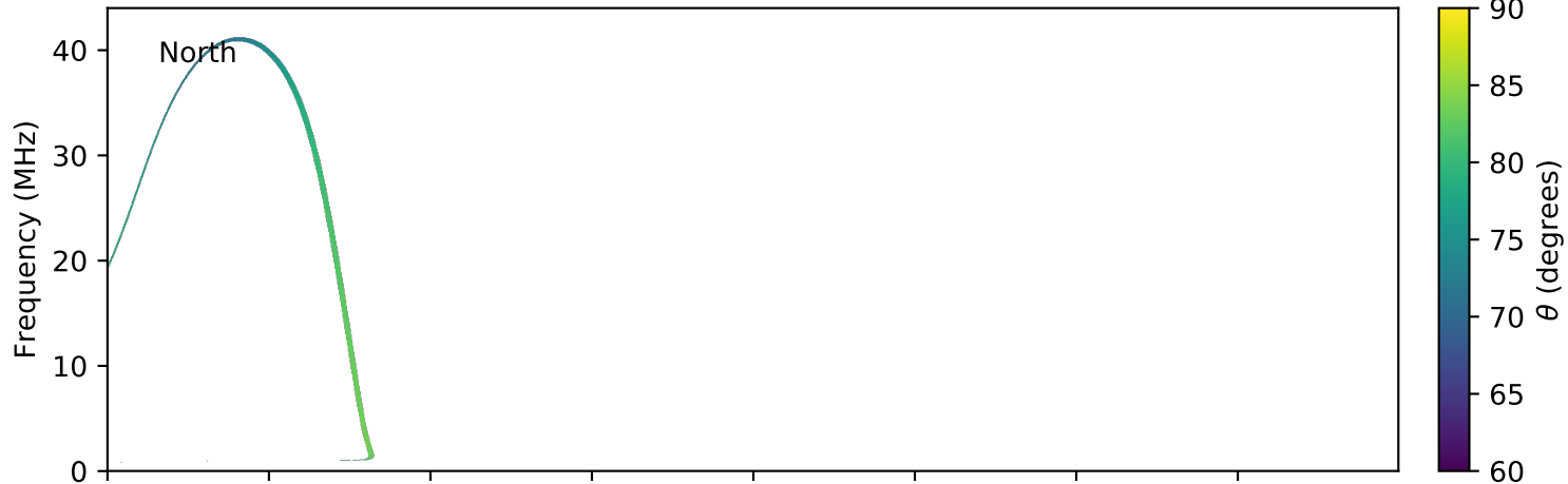
expres_earth_jupiter_io_jrm09_lossc-wid1deg_3kev_20180124_v01.cdf
