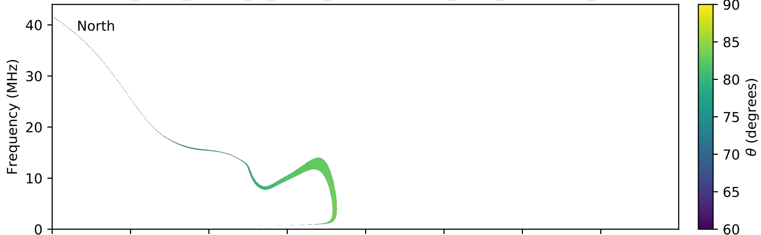
expres_earth_jupiter_io_jrm09_lossc-wid1deg_3kev_20180122_v01.cdf
