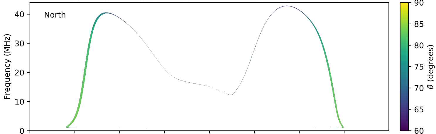
expres_earth_jupiter_io_jrm09_lossc-wid1deg_3kev_20180118_v01.cdf
