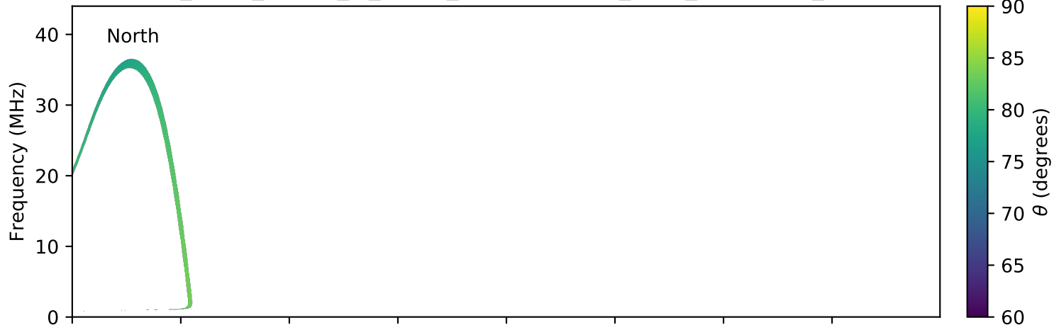
expres_earth_jupiter_io_jrm09_lossc-wid1deg_3kev_20180117_v01.cdf
