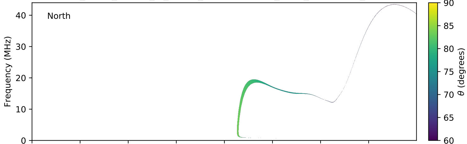
expres_earth_jupiter_io_jrm09_lossc-wid1deg_3kev_20180114_v01.cdf
