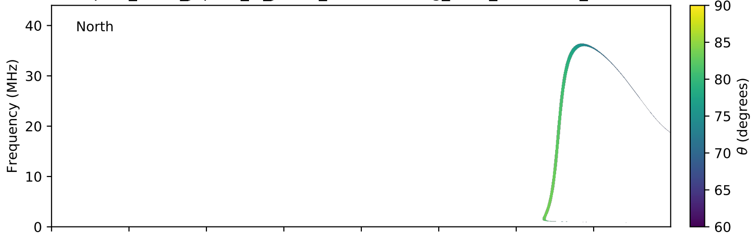
expres_earth_jupiter_io_jrm09_lossc-wid1deg_3kev_20180112_v01.cdf
