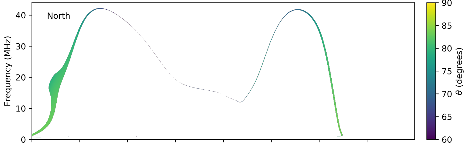
expres_earth_jupiter_io_jrm09_lossc-wid1deg_3kev_20180111_v01.cdf
