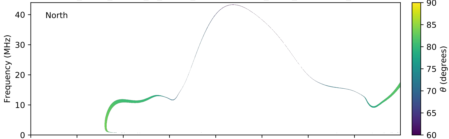
expres_earth_jupiter_io_jrm09_lossc-wid1deg_3kev_20180109_v01.cdf
