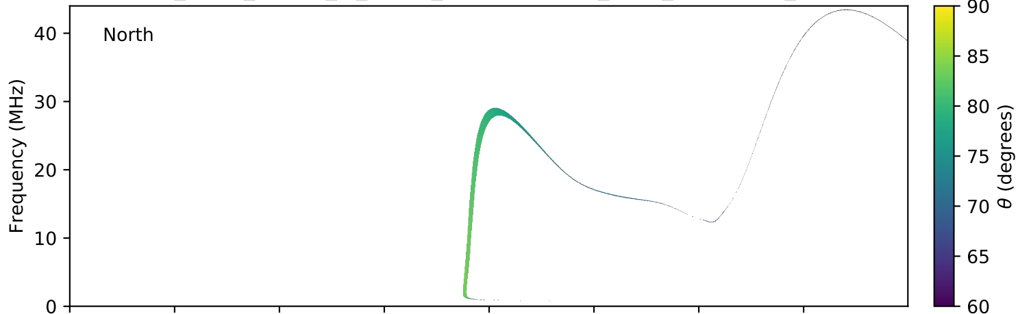
expres_earth_jupiter_io_jrm09_lossc-wid1deg_3kev_20180107_v01.cdf
