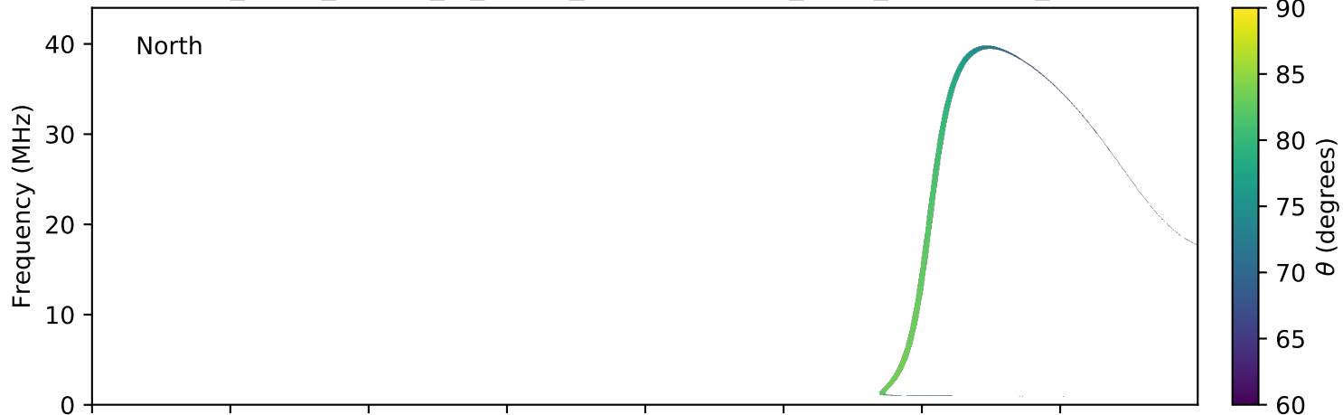
expres_earth_jupiter_io_jrm09_lossc-wid1deg_3kev_20180105_v01.cdf
