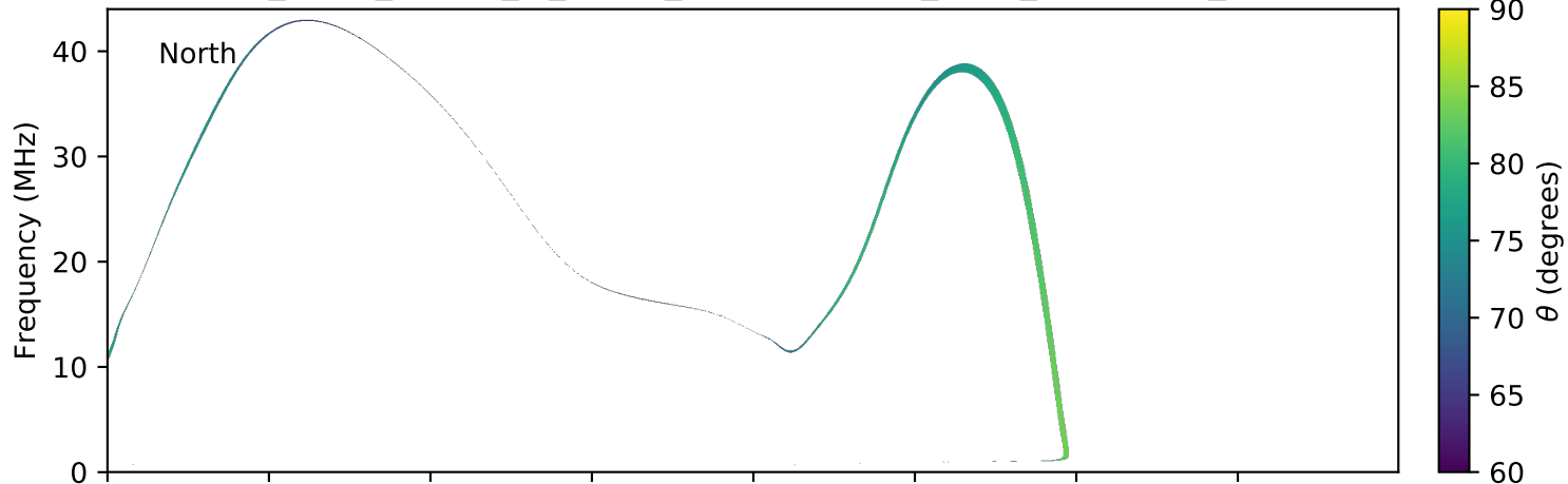
expres_earth_jupiter_io_jrm09_lossc-wid1deg_3kev_20180104_v01.cdf
