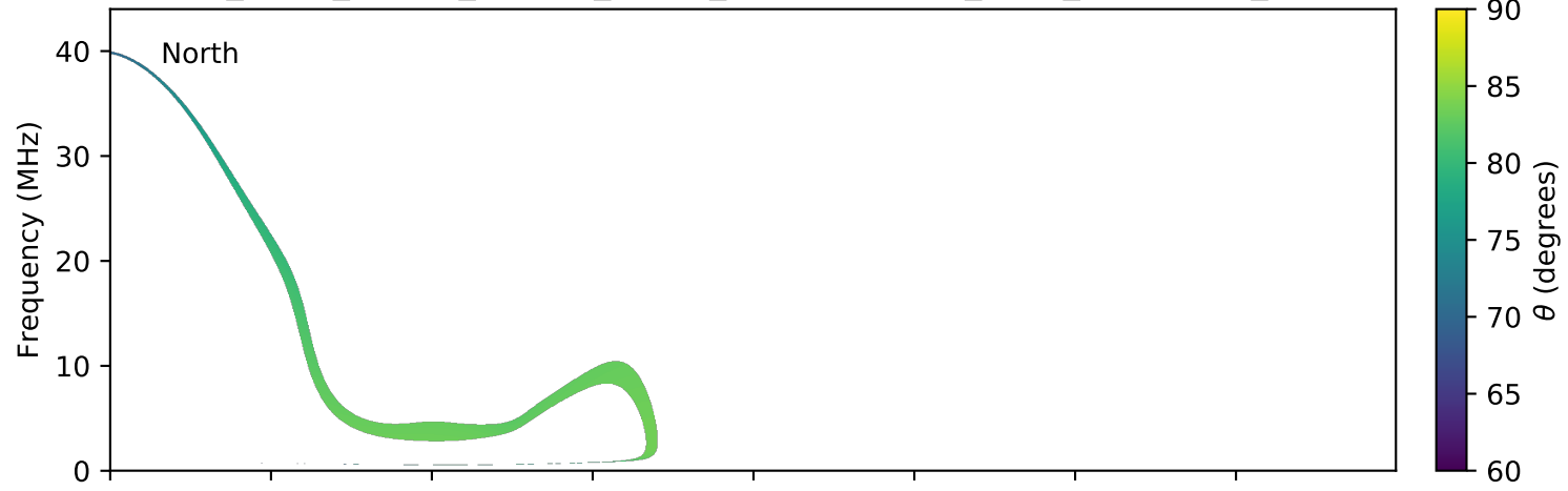
expres_earth_jupiter_europa_jrm09_lossc-wid1deg_3kev_20180127_v01.cdf
