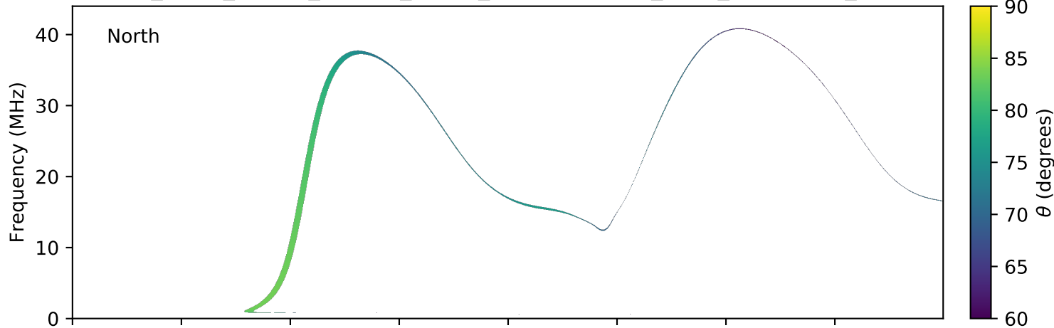
expres_earth_jupiter_europa_jrm09_lossc-wid1deg_3kev_20180115_v01.cdf
