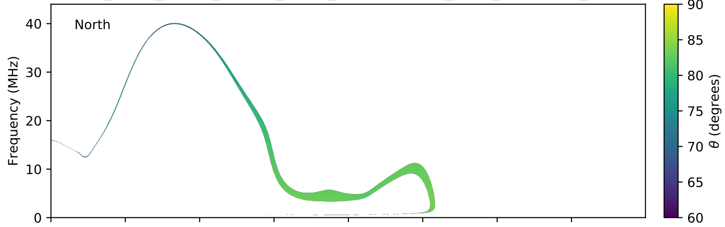
expres_earth_jupiter_europa_jrm09_lossc-wid1deg_3kev_20180109_v01.cdf
