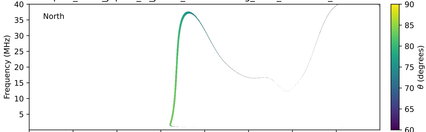
expres_earth_jupiter_io_jrm33_lossc-wid1deg_3kev_20171231_v11.cdf
