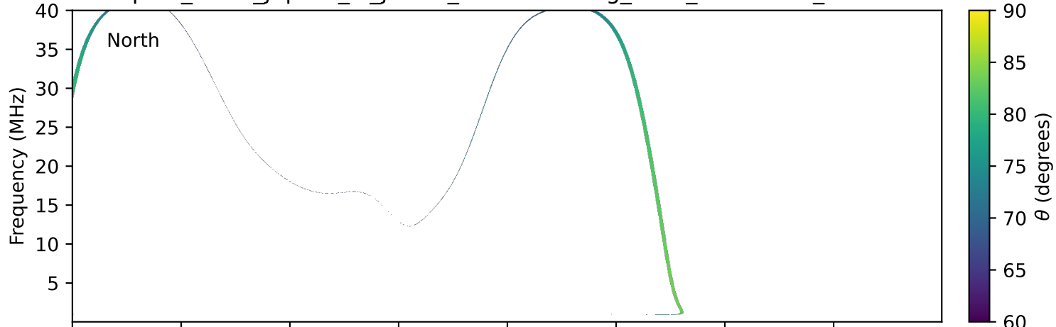
expres_earth_jupiter_io_jrm33_lossc-wid1deg_3kev_20171226_v11.cdf
