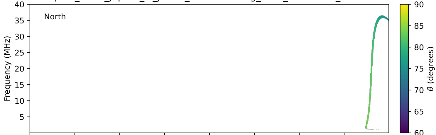
expres_earth_jupiter_io_jrm33_lossc-wid1deg_3kev_20171216_v11.cdf
