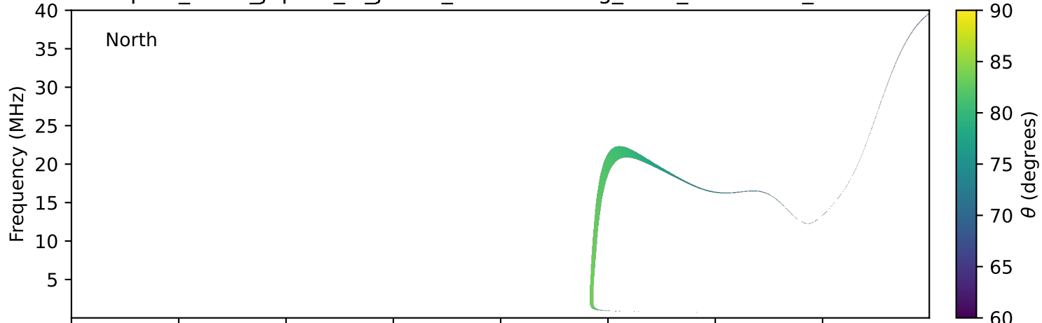
expres_earth_jupiter_io_jrm33_lossc-wid1deg_3kev_20171211_v11.cdf
