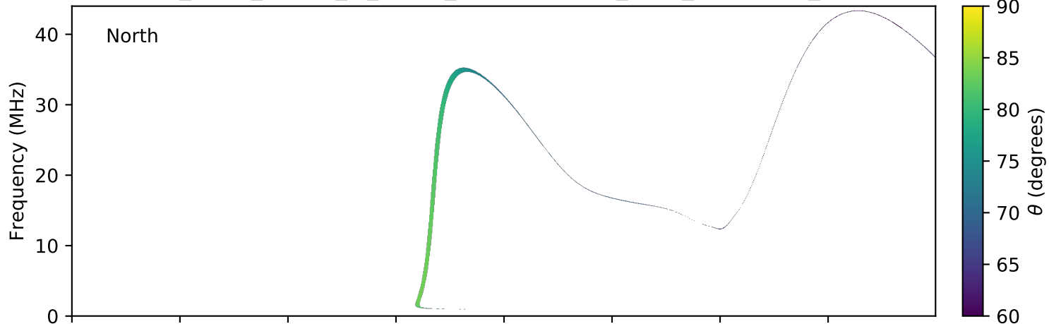
expres_earth_jupiter_io_jrm09_lossc-wid1deg_3kev_20171231_v01.cdf
